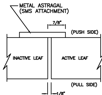
FLAT METAL ASTRAGAL
