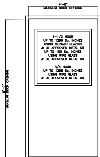
FIRE RATED SINGLE DOOR ONLY 1 LOUVER/WINDOW OPENING PER LEAF
