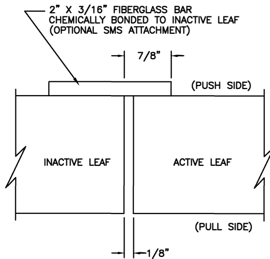
FLAT FIBERGLASS ASTRAGAL (NON-RATED DOORS)
