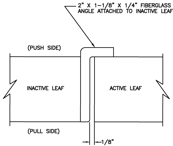
INTEGRAL FIBERGLASS ASTRAGAL (RATED DOORS)
