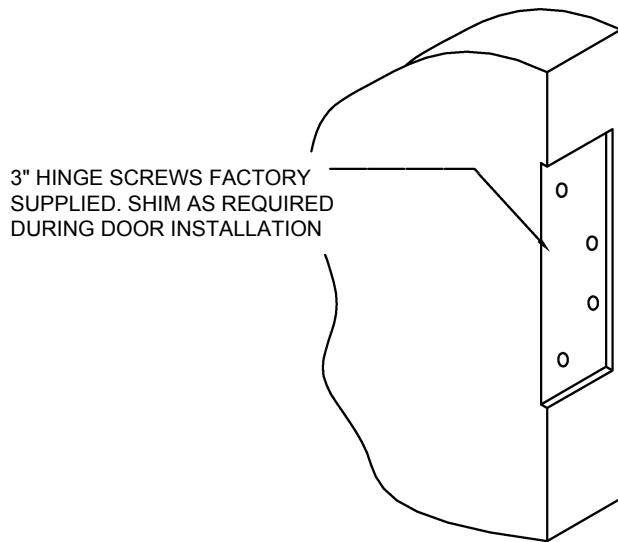
HINGE DETAIL
