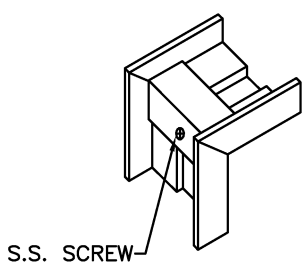
STANDARD KD KNOCK DOWN NO EXPOSED FASTENERS
