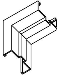
OPTION WF CHEMICALLY WELDED FACE
