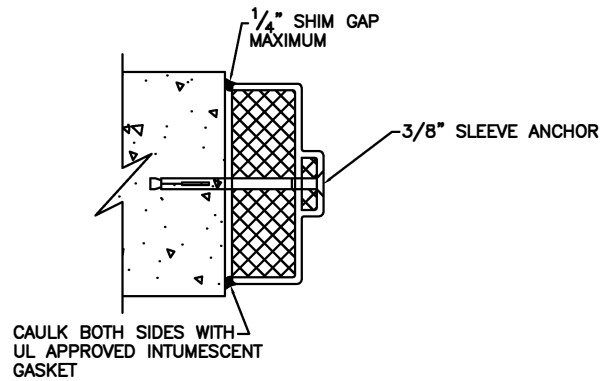
FIRE RATED FRAME ANCHOR
