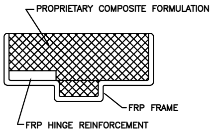
FIRE RATED FRAME SECTION
