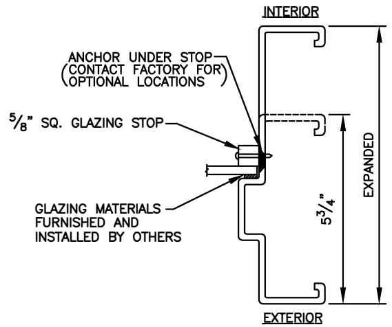
GLAZING PLACEMENT
