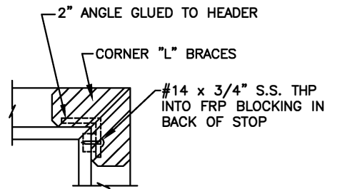
STANDARD KD CONNECTION
